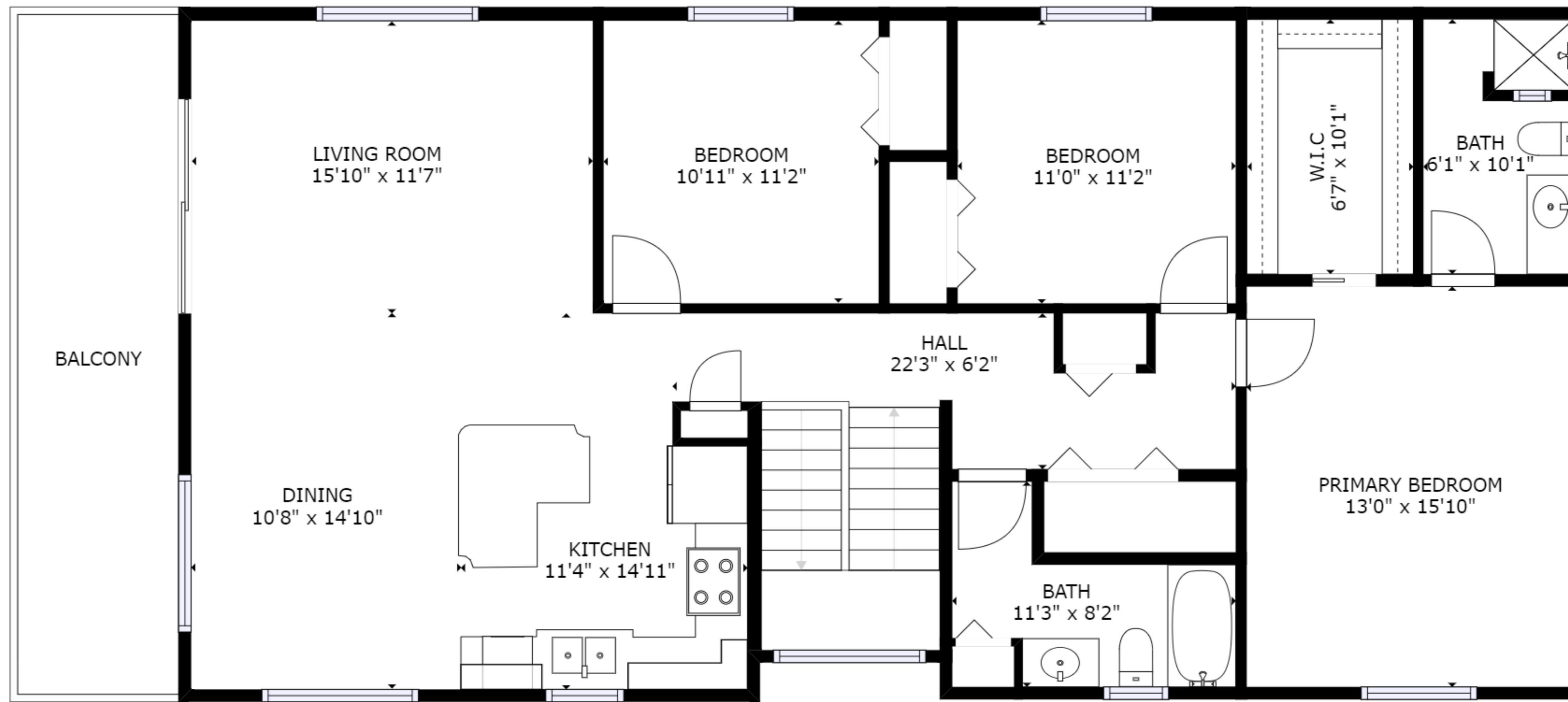
FLOOR 2
